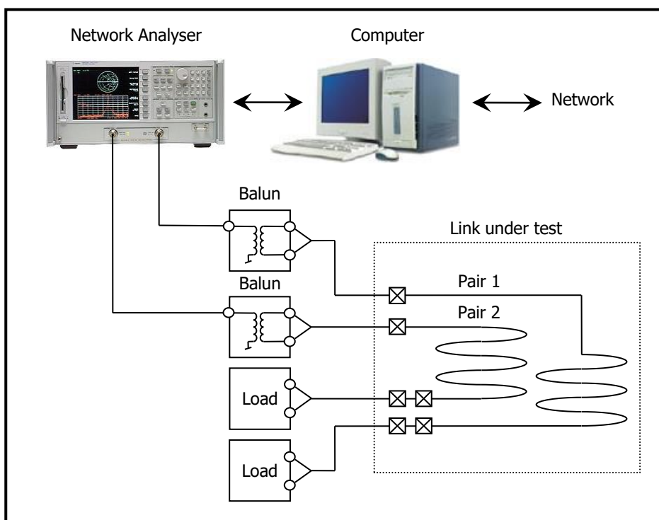
Figure 5. Test set-up for near end cross talk measurements.
