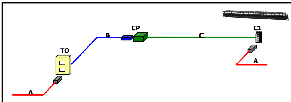
Figure 1. Definition of link (3 connector model).
