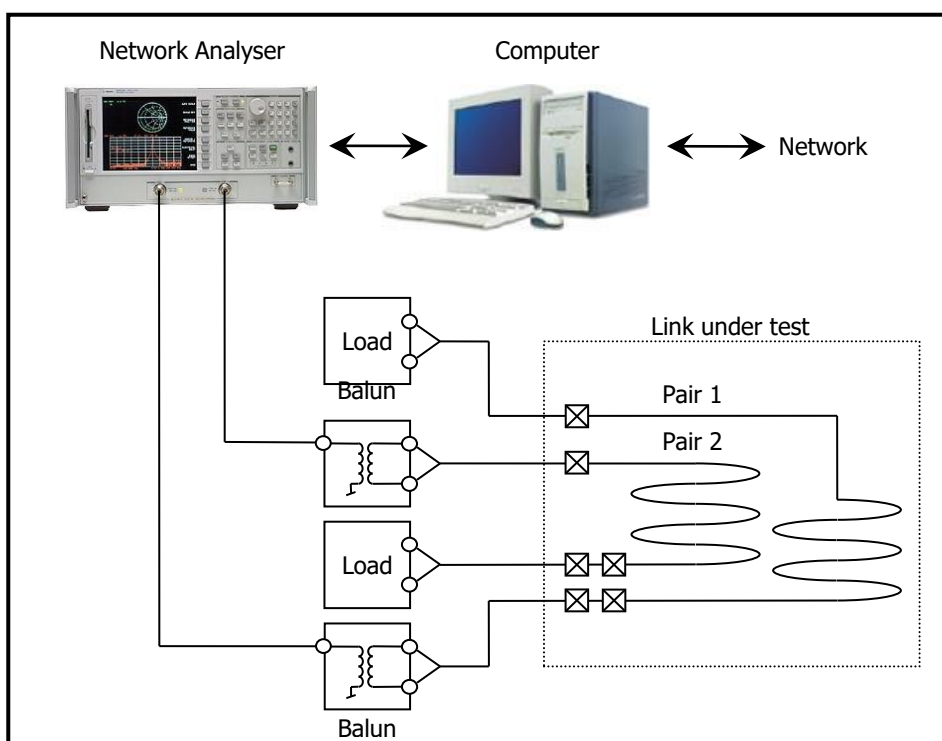
Figure 6. Test set-up for far end crosstalk measurements.
