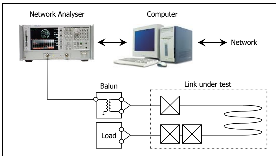
Figure 4. Test set-up for return loss measurements.
